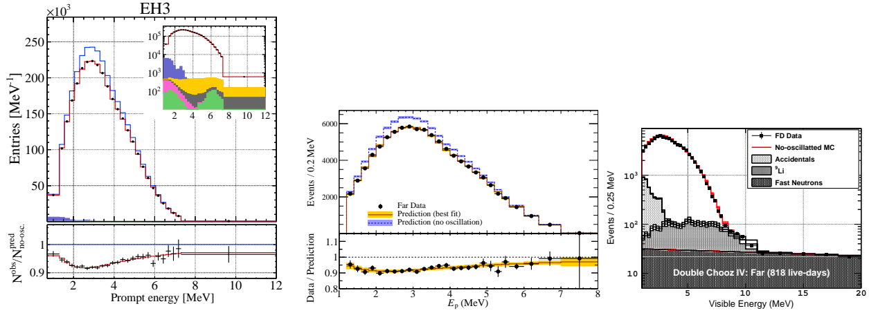
Figure 14.8: Energy spectra for prompt events at the far detectors for Daya Bay [146], RENO [137], and Double Chooz [138].
