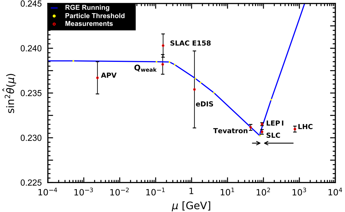
Figure 10.2: Scale dependence of the weak mixing angle defined in the \overline{\text{MS}} scheme [39, 83] (for the scale dependence in a mass-dependent renormalization scheme, see Ref. [82]). The minimum of the curve corresponds to \mu = M_W , below which we switch to an effective theory with the W^\pm bosons integrated out, and where the \beta -function for \hat{s}^2(\mu) changes sign. At M_W and each fermion mass there are also discontinuities arising from scheme dependent matching terms, which are necessary to ensure that the various effective field theories within a given loop order describe the same physics. However, in the \overline{\text{MS}} scheme these are very small numerically and barely visible in the figure provided one decouples quarks at \mu = \hat{m}_q(\hat{m}_q) . The width of the curve exceeds the theory uncertainty from strong interaction effects which at low energies is at the level of \pm 2 \times 10^{-5} [39]. The Tevatron and LHC measurements are strongly dominated by invariant masses of the final-state di-lepton pair of \mathcal{O}(M_Z) and can thus be considered as additional Z pole data points. For clarity we displayed the Tevatron and LHC points horizontally to the left and right, respectively.
