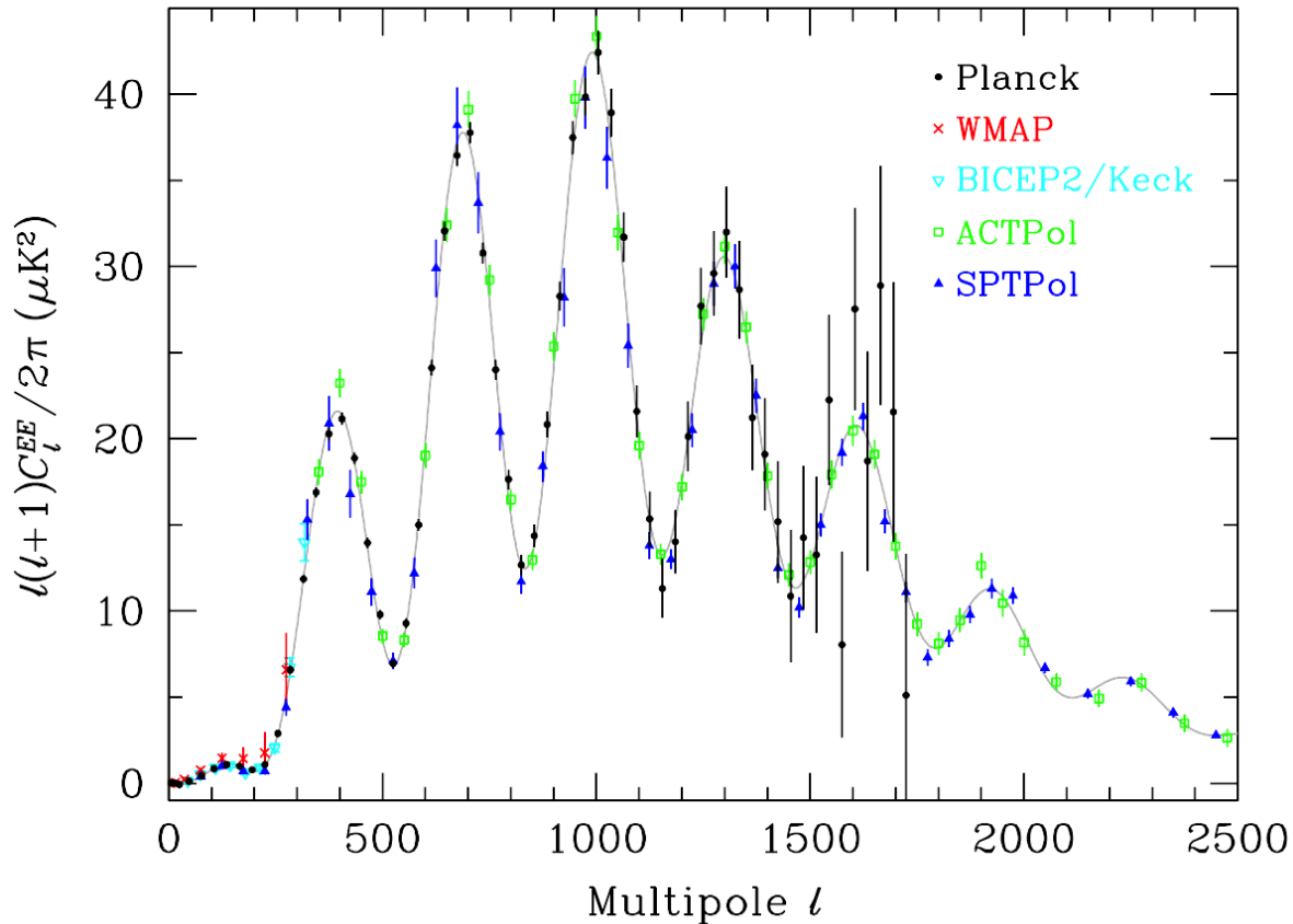
Figure 29.4: Power spectrum of E -mode polarization from Planck , together with WMAP , BICEP2/Keck , ACTPol , and SPTPol . Note that some band-powers with larger uncertainties have been omitted and that the unbinned Planck low- \ell data have been binned here. Also plotted is the best-fit theoretical model from Planck temperature, polarization, and lensing data.
