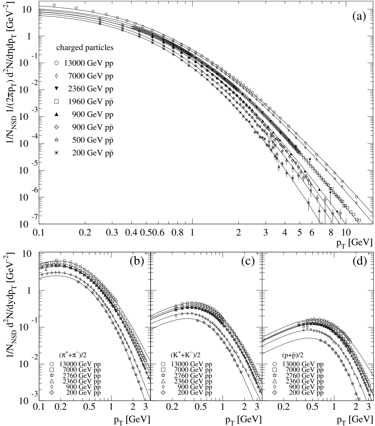
Figure 19.11: (a) Selection of inclusive charged-particle transverse momentum spectra [114, 117, 119, 121, 160, 202, 203], normalized to the non-single diffractive cross section (NSD). (b)-(d) Selection of identified charged-particle transverse momentum spectra [204–209] normalized to the NSD cross section. All spectra are scaled to the NSD cross-section using measurements of total, inelastic, elastic, single, or non-single diffractive cross sections from [210–214, 214–216]. The overall normalization uncertainty of about 3% is not shown. Superimposed are fits of the Tsallis distribution in Eq. (19.13).
