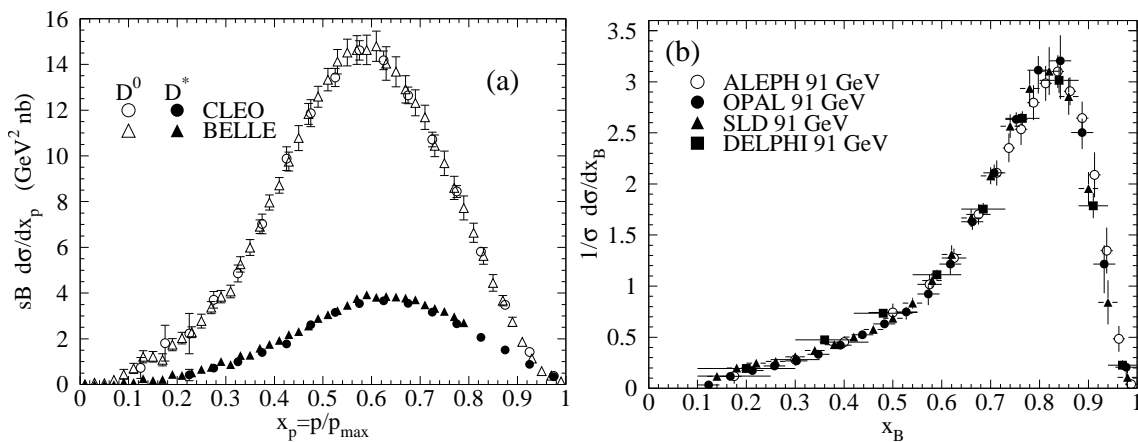
Figure 19.12: (a) Efficiency-corrected inclusive cross-section measurements for the production of D^0 and D^{*+} in e^+e^- measurements at \sqrt{s} \approx 10.6 GeV, excluding B decay products [272] [273]. (b) Measured e^+e^- fragmentation function of b quarks into B hadrons at \sqrt{s} \approx 91 GeV [274].
