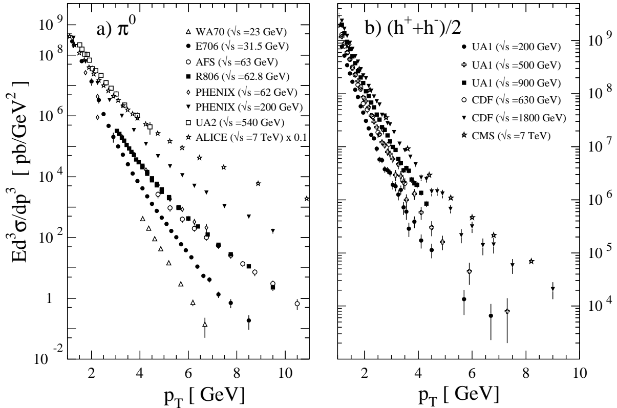
Figure 19.10: Selection of inclusive (a) \pi^0 and (b) charged-hadron production data from pp [118, 154–159] and p\bar{p} [114, 160, 161] collisions.
