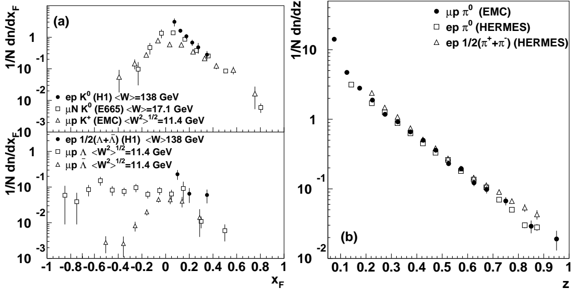
Figure 19.9: (a) 1/N \cdot dn/dx_F for identified strange particles in DIS at various values of W [148–150]. (b) 1/N \cdot dn/dz for measurements of pions in fixed-target DIS experiments [151–153].
