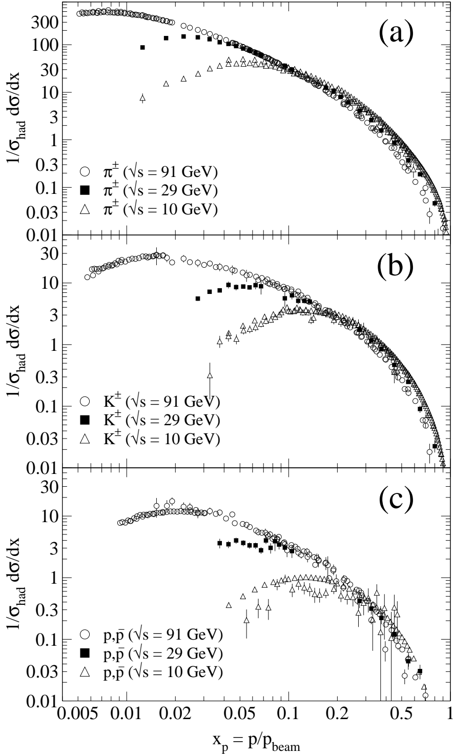
Figure 19.8: Scaled momentum spectra of (a) \pi^\pm , (b) K^\pm , and (c) p, \bar{p} at \sqrt{s} = 10, 29, and 91 GeV [24, 26, 85, 146, 147].
