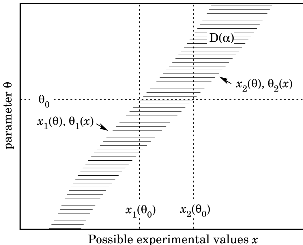
Figure 39.3: Construction of the confidence belt (see text).
