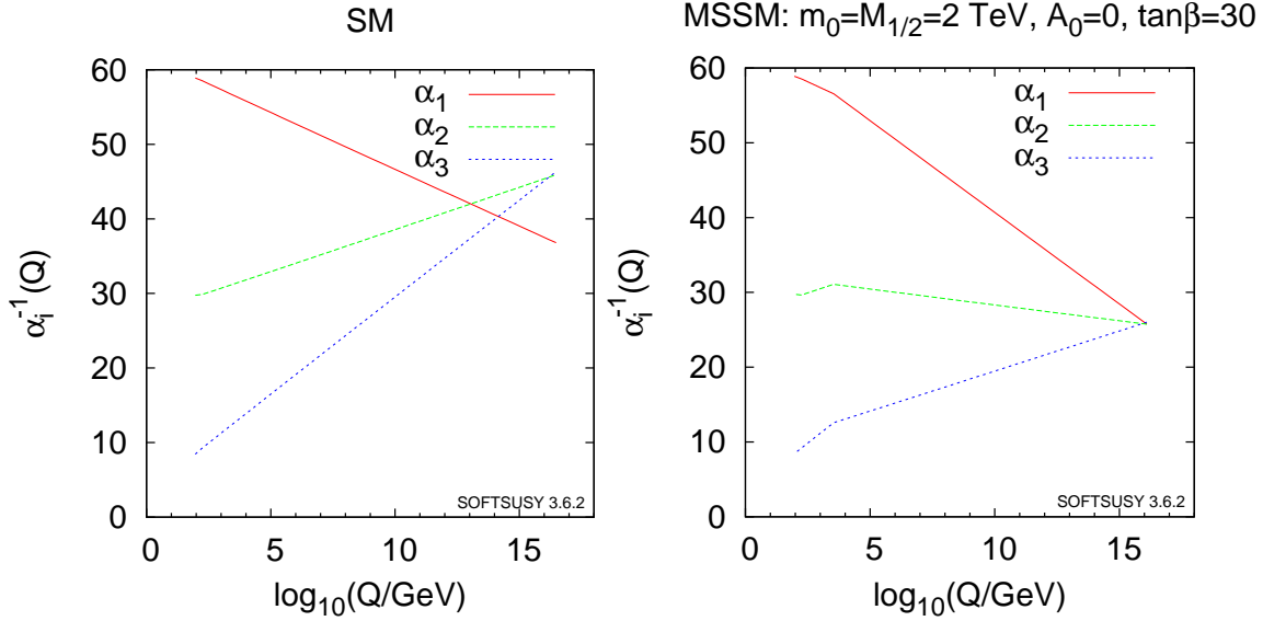
Figure 115.1: Running couplings in SM and MSSM using two-loop RG evolution. The SUSY threshold at 2 TeV is clearly visible on the MSSM side. (We thank Ben Allanach for providing the plots created using SOFTSUSY [61].)
