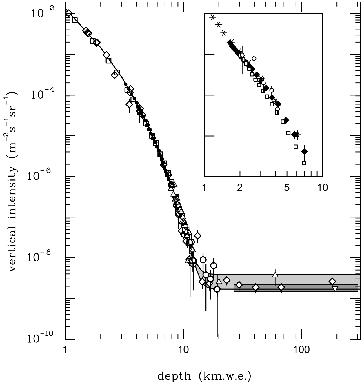
Figure 29.7: Vertical muon intensity vs depth (1 km.w.e. = 10^5 g cm ^{-2} of standard rock). The experimental data are from: \diamond : the compilations of Crouch [73], \square : Baksanu [74], \circ : LVD [75], \bullet : MACRO [76], \blacksquare : Frejus [77], and \triangle : SNO [78]. The shaded area at large depths represents neutrino-induced muons of energy above 2 GeV. The upper line is for horizontal neutrino-induced muons, the lower one for vertically upward muons. Darker shading shows the muon flux measured by the SuperKamiokande experiment. The inset shows the vertical intensity curve for water and ice published in Refs. [79–82]. Additional data extending to slant depths of 13 km are available in [83].
