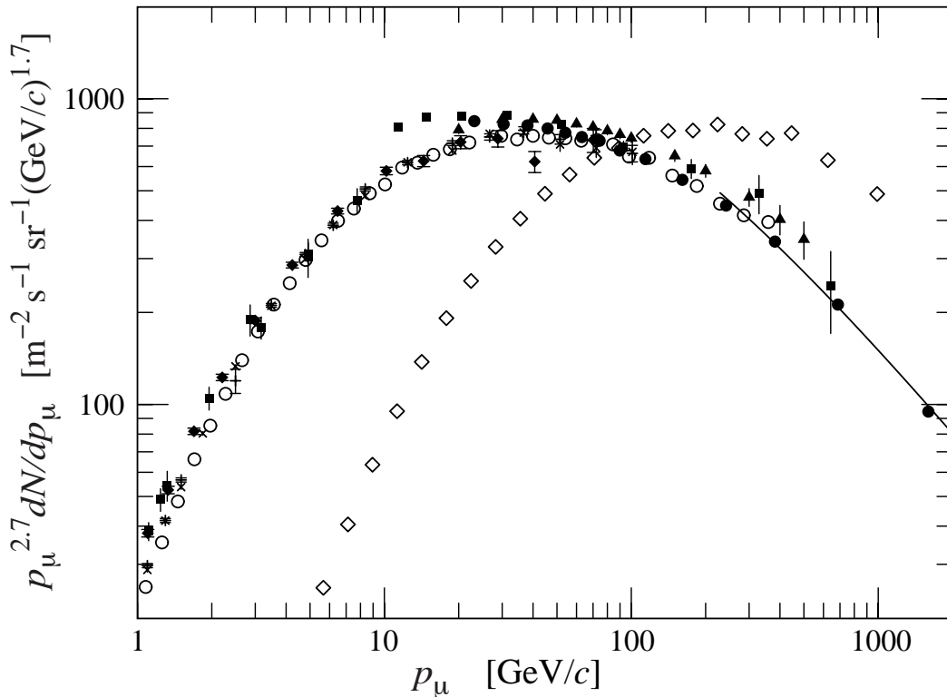
Figure 29.5: Spectrum of muons at \theta = 0^\circ ( \blacklozenge [56], \blacksquare [60], \blacktriangledown [61], \blacktriangle [62], \times , + [58], \circ [51], and \bullet [59] and \theta = 75^\circ \diamond [63]). The line plots the result from Eq. (29.4) for vertical showers.
