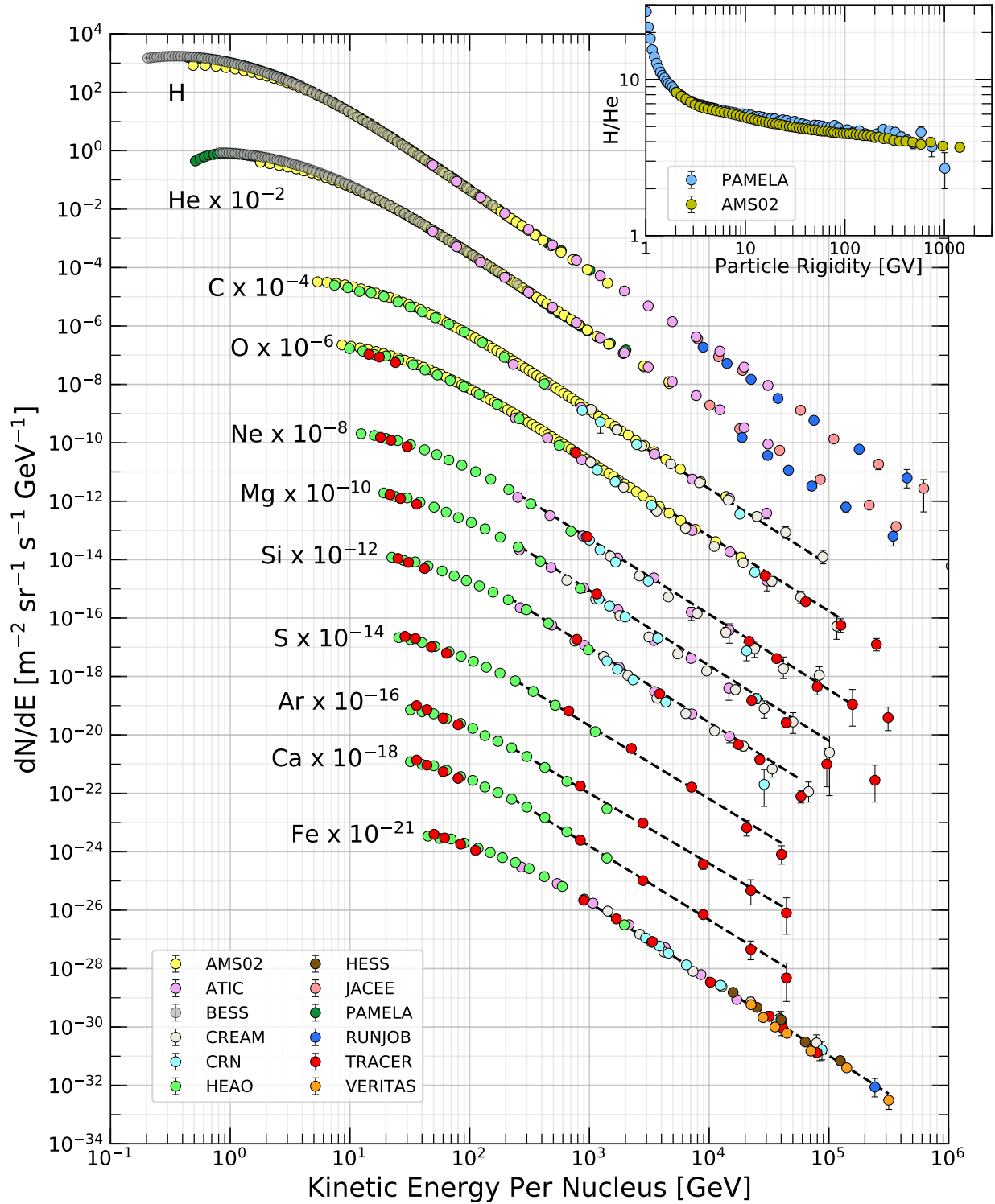
Figure 29.1: Fluxes of nuclei of the primary cosmic radiation in particles per energy-per-nucleus are plotted vs energy-per-nucleus using data from Refs. [1–13] The inset shows the H/He ratio as a function of rigidity [1, 3].
