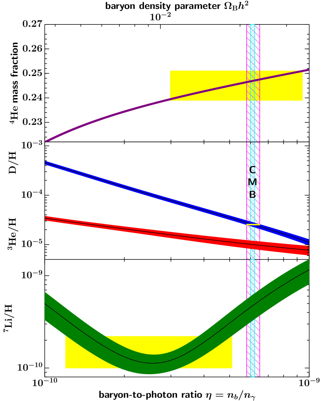
Figure 23.1: The primordial abundances of {}^4\text{He} , D, {}^3\text{He} , and {}^7\text{Li} as predicted by the standard model of Big-Bang nucleosynthesis — the bands show the 95% CL range [47]. Boxes indicate the observed light element abundances. The narrow vertical band indicates the CMB measure of the cosmic baryon density, while the wider band indicates the BBN D+ {}^4\text{He} concordance range (both at 95% CL).
