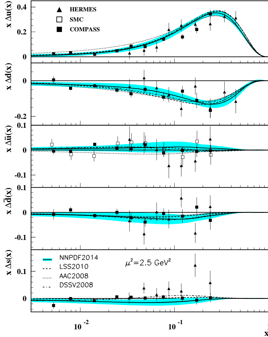
Figure 18.3: Distributions of x times the polarized parton distributions \Delta q(x) (where q = u, d, \bar{u}, \bar{d}, s ) using the NNPDF2014 [17], AAC2008 [18], DSSV2008 [19], and LSS2010 [20] parameterizations at a scale \mu^2 = 2.5 \text{ GeV}^2 , showing the blue-shaded error corridor of the NNPDF2014 set. (SMC [23] and COMPASS [24,25]) deep inelastic scattering given at Q^2 = 2.5 \text{ GeV}^2 . The SMC results were extracted under the assumption that \Delta \bar{u}(x) = \Delta \bar{d}(x) .
