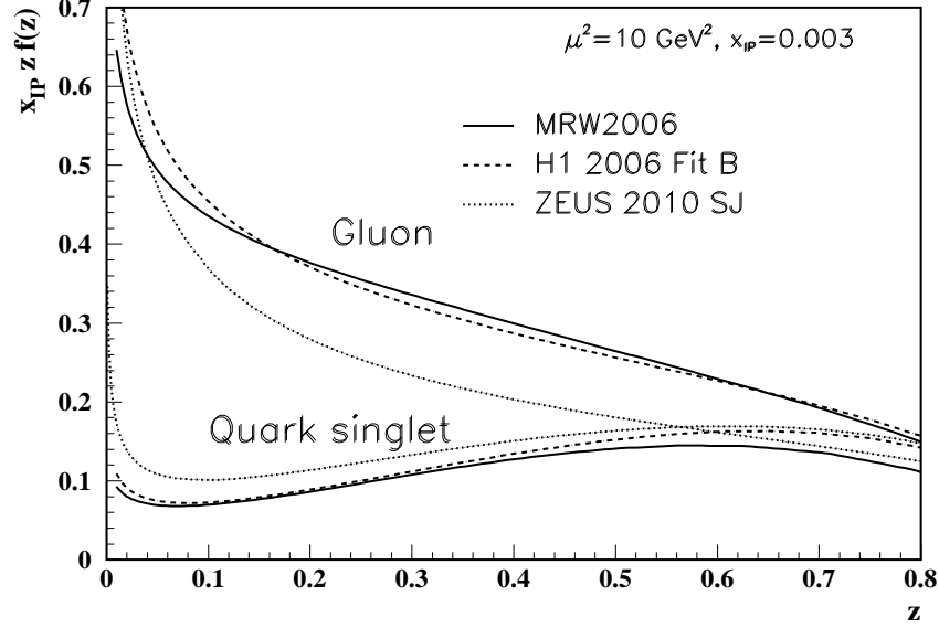
Figure 18.6: Diffractive parton distributions, x_{IP} z f_{a/p}^D , obtained from fitting to the ZEUS data with Q^2 > 5 \text{ GeV}^2 [112], H1 data with Q^2 > 8.5 \text{ GeV}^2 assuming Regge factorization [113], and from MRW2006 [114] using a more perturbative QCD approach [114]. Only the Pomeron contributions are shown and not the secondary Reggeon contributions, which are negligible at the value of x_{IP} = 0.003 chosen here. The H1 2007 Jets distribution [115] is similar to H1 2006 Fit B.
