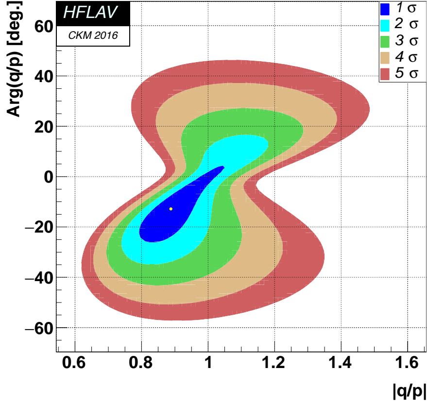
Figure 82.2: Two-dimensional 1\sigma - 5\sigma contours for (|q/p|, \text{Arg}(q/p)) from measurements of D^0 \rightarrow K^{(*)+} \ell \nu , h^+ h^- , K^+ \pi^- , K^+ \pi^- \pi^0 , K^+ \pi^- \pi^+ \pi^- , K_S^0 \pi^+ \pi^- , K_S^0 K^+ K^- , and \pi^+ \pi^- \pi^0 decays, and double-tagged branching fractions measured at the \psi(3770) resonance (from HFLAV [9]).
