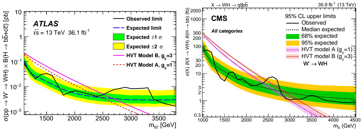
Figure 107.2: Upper limits at 95% CL on W' production cross section times branching fraction into a W and a SM Higgs boson, from [41] (left) and [44] (right).
