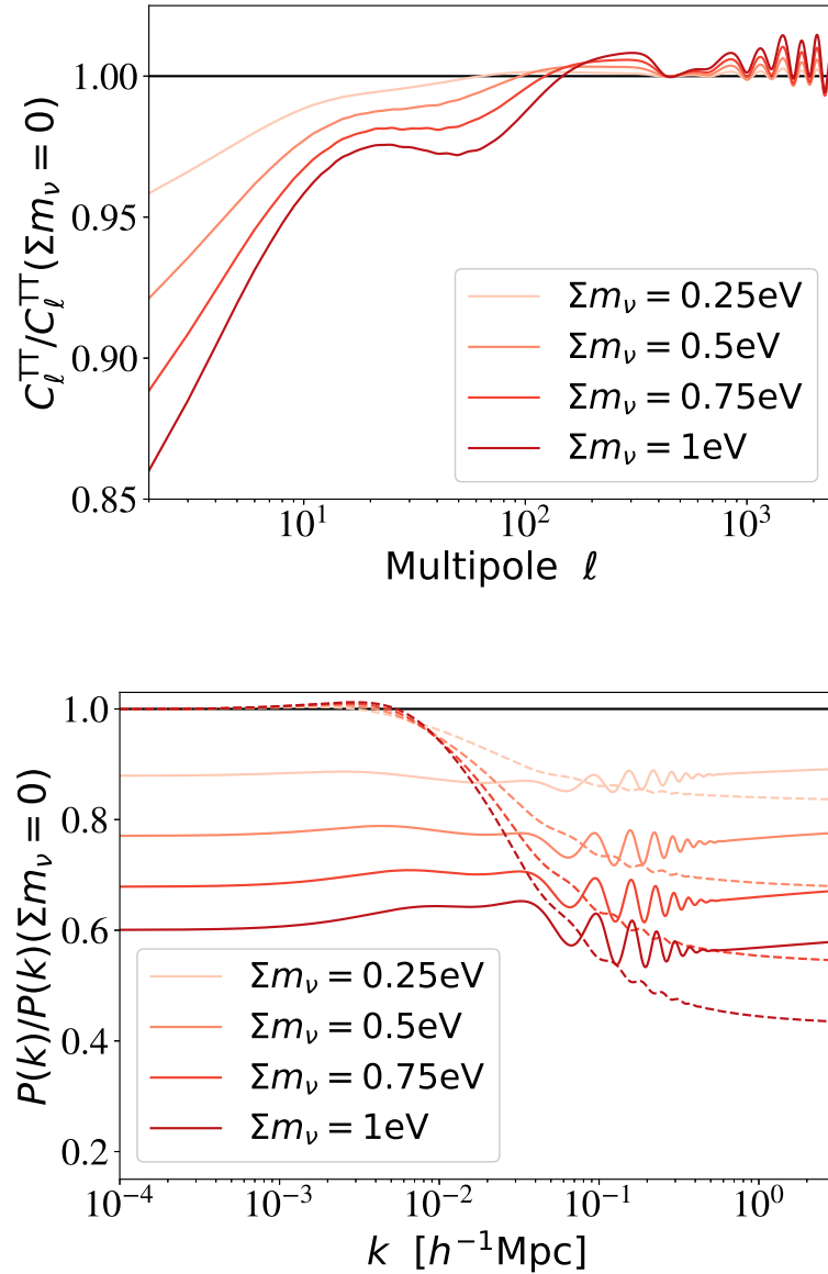
Figure 25.2: Ratio of the CMB C_\ell^{TT} and matter power spectrum P(k) (computed for each model in units of (h^{-1}\text{Mpc})^3 ) for different values of \Sigma m_\nu over those of a reference model with massless neutrinos. In order to minimize and better characterise the effect of \Sigma m_\nu on the CMB, the parameters that are kept fixed are \omega_b , \omega_c , \tau , the angular scale of the sound horizon \theta_s and the primordial spectrum parameters (solid lines). This implies that we are increasing the Hubble parameter h as a function of \Sigma m_\nu . For the matter power spectrum, in order to single out the effect of neutrino free-streaming on P(k) , the dashed lines show the spectrum ratio when \{\omega_m, \omega_b, \Omega_\Lambda\} are kept fixed. For comparison, the error on P(k) is of the order of 5% with current observations, and the fractional C_\ell errors are of the order of 1/\sqrt{\ell} at low \ell .
