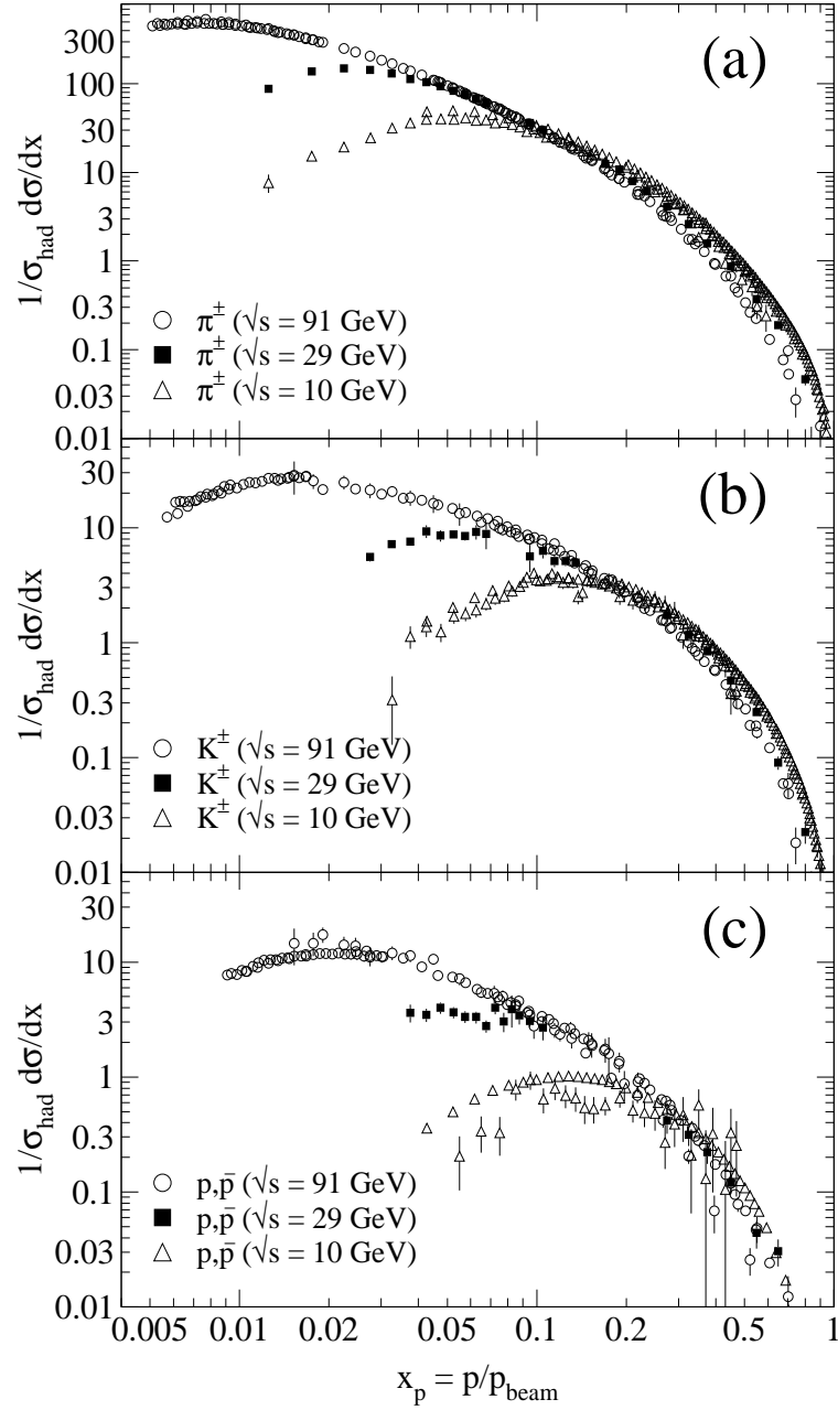
Figure 20.8: Scaled momentum spectra of (a) \pi^\pm , (b) K^\pm , and (c) p/\bar{p} at \sqrt{s} = 10, 29, \text{ and } 91 GeV [42–44,87,155,156].
