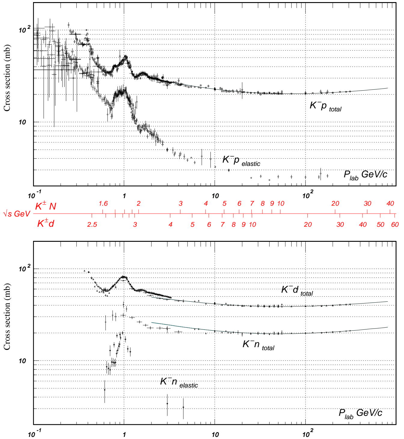
Figure 49.9D14: Total and elastic cross sections for K^-p and K^-d (total only), and K^-n collisions as a function of laboratory beam momentum and total center-of-mass energy. Corresponding data files may be found at http://pdg.lbl.gov/xsect/contents.html (Courtesy of the COMPAS Group, IHEP, Protvino, September 2013.)
