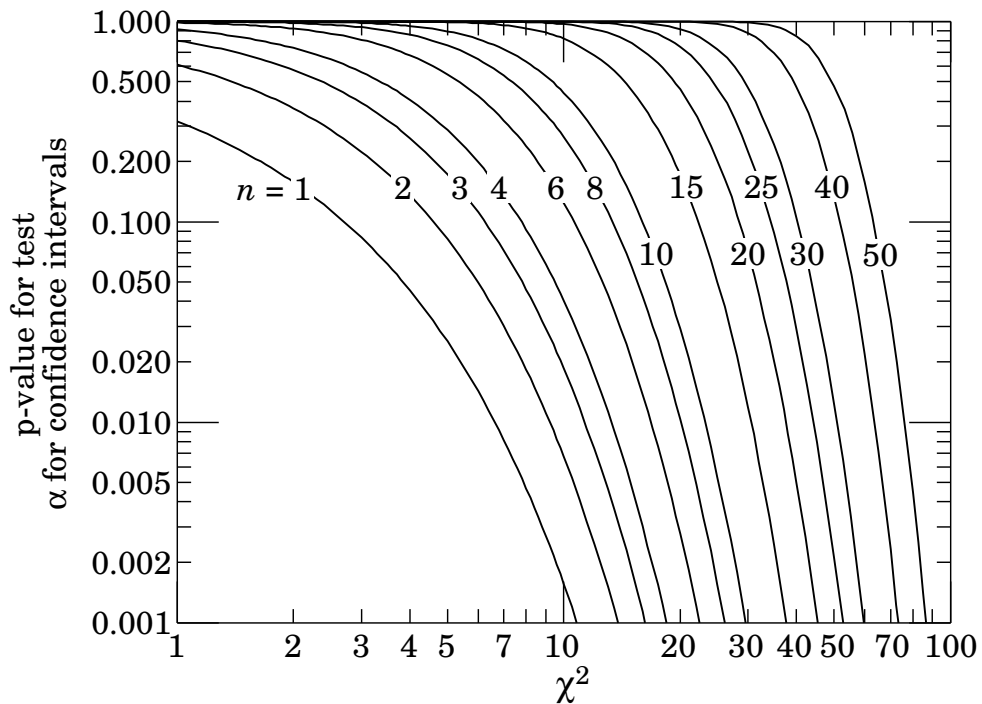
Figure 37.1: One minus the \chi^2 cumulative distribution, 1 - F(\chi^2; n) , for n degrees of freedom. This gives the p -value for the \chi^2 goodness-of-fit test as well as one minus the coverage probability for confidence regions (see Sec. 37.4.2.2).
