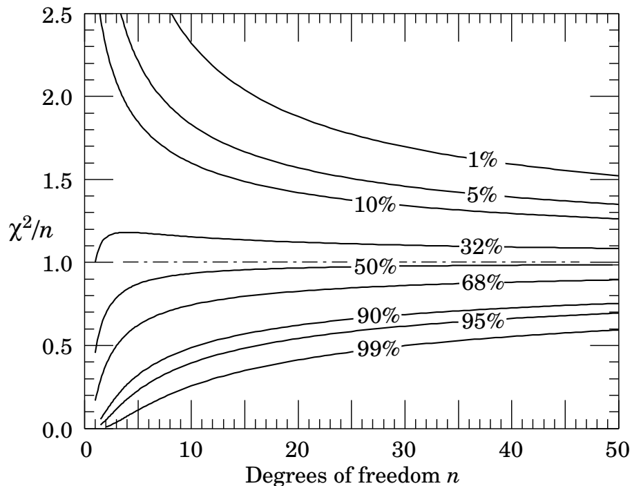
Figure 37.2: The ‘reduced’ \chi^2 , equal to \chi^2/n , for n degrees of freedom. The curves show as a function of n the \chi^2/n that corresponds to a given p -value.
