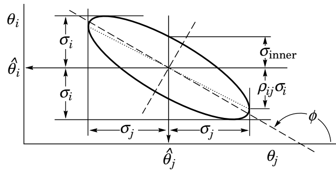
Figure 37.5: Standard error ellipse for the estimators \hat{\theta}_i and \hat{\theta}_j . In this case the correlation is negative.
