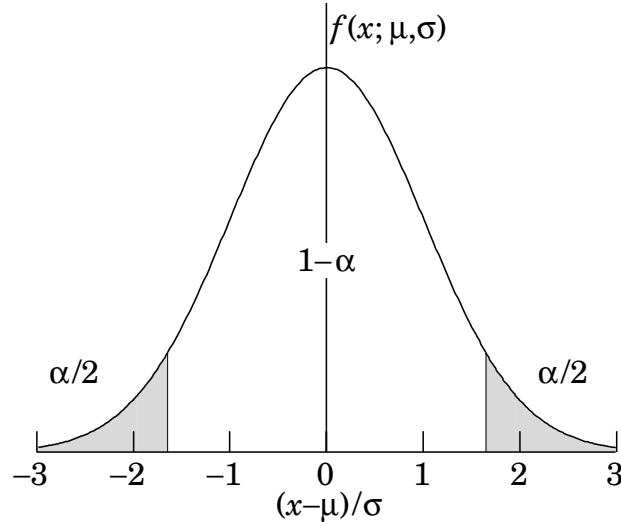
Figure 37.4: Illustration of a symmetric 90% confidence interval (unshaded) for a measurement of a single quantity with Gaussian errors. Integrated probabilities, defined by \alpha = 0.1 , are as shown.
