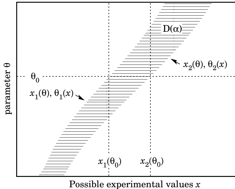
Figure 37.3: Construction of the confidence belt (see text).
