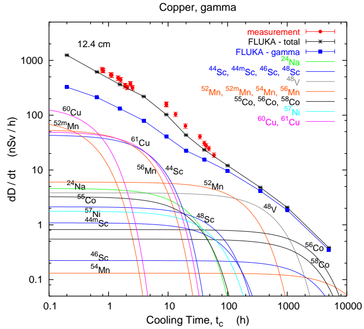
Figure 34.5: Contribution of individual gamma-emitting nuclides to the total dose rate at 12.4 cm distance to an activated copper sample [12].
