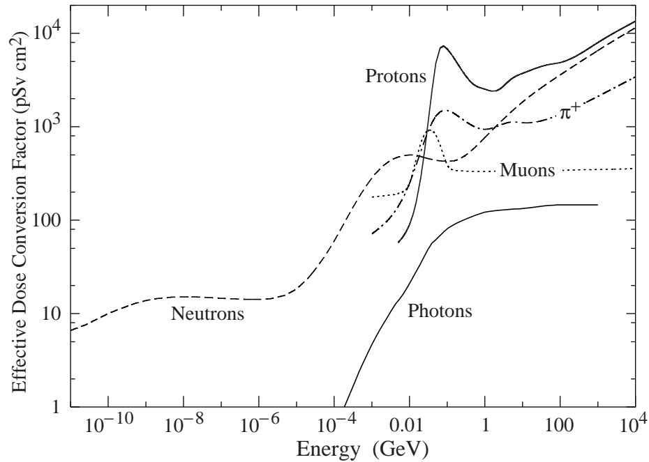
Figure 34.1: Fluence to effective dose conversion coefficients for anterior-posterior irradiation and various particles [3].
