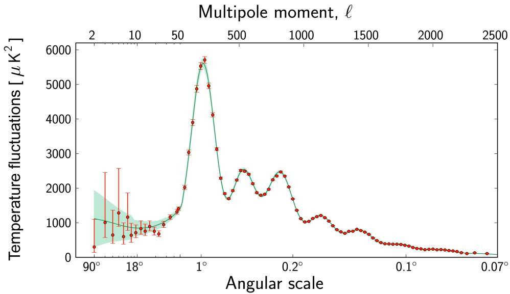
Figure 23.1: The angular power spectrum of the CMB temperature anisotropies from Planck , from Ref. 1. Note the x -axis switches from logarithmic to linear at \ell = 50 . The solid line shows the prediction from the best-fitting \Lambda CDM model and the band indicates the cosmic variance uncertainty. [Figure courtesy ESA/ Planck Collaboration.]
