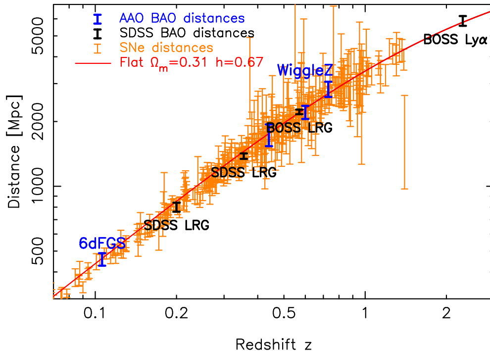
Figure 23.2: The cosmic distance scale with redshift. This modern version of the ‘Hubble Diagram’ combines data from SN Ia as standard candles and BAO as standard rulers in the LRG SDDS, BOSS, 6dFGRS, and WiggleZ galaxy surveys and from the BOSS Lyman-alpha at high redshift. [Figure courtesy of C. Blake, based on Ref. 33.]
