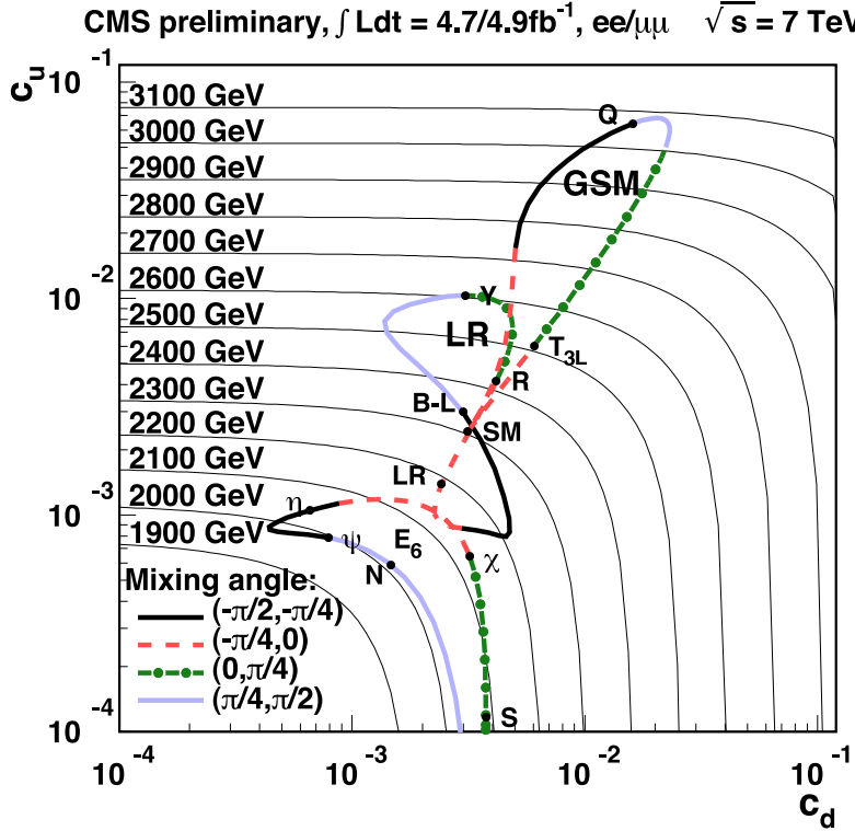
Figure 2: CMS results from Ref. 35. Limits in the c_u^\ell - c_d^\ell plane ( \ell = e or \mu ) are shown as thin lines for certain M_{Z'} values. For specific sets of charges (described in Ref. 5), parametrized by a mixing angle, the mass limit is given by the intersection of the thick and thin lines.
