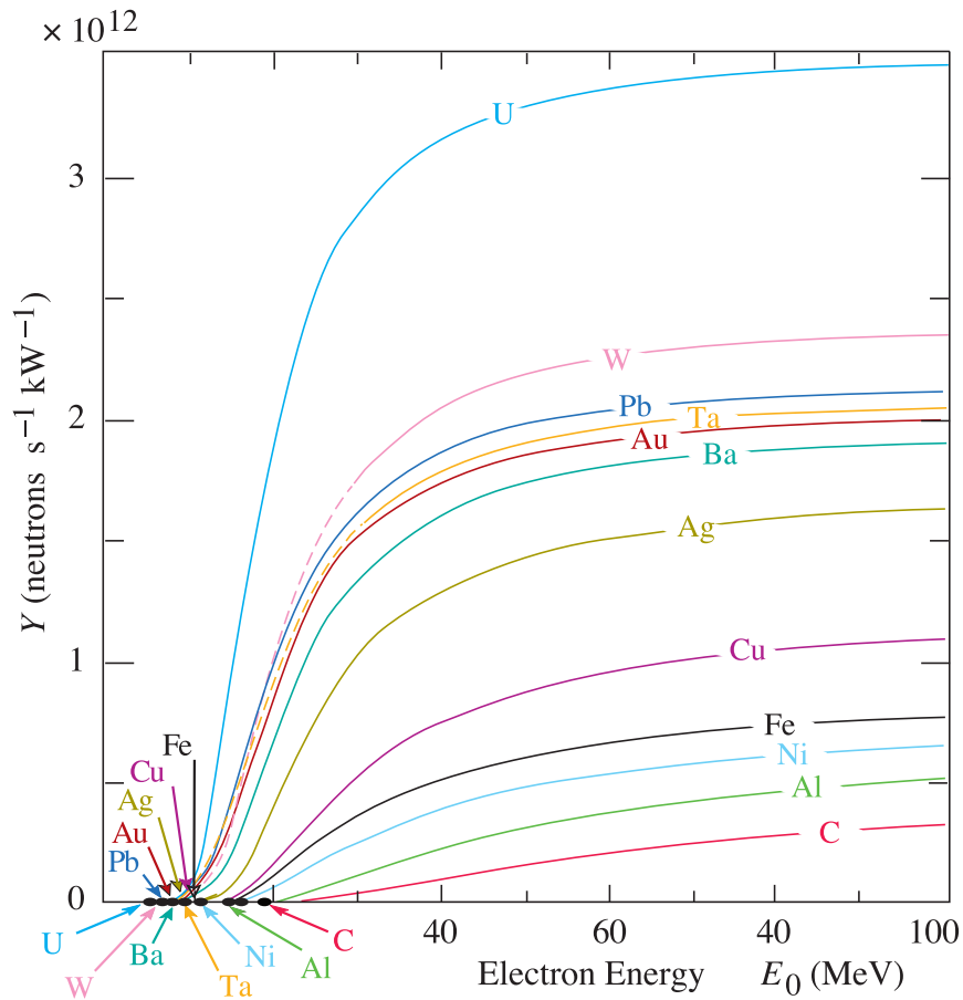
Figure 33.2: Neutron yields from semi-infinite targets per kW of electron beam power, as a function of the electron beam energy, disregarding target self-shielding [6].
