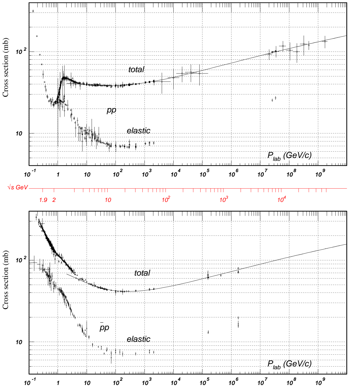
Figure 49.9D11: Total and elastic cross sections for pp and \bar{p}p collisions as a function of laboratory beam momentum and total center-of-mass energy. Corresponding data files may be found at http://pdg.lbl.gov/xsect/contents.html (Courtesy of the COMPAS group, IHEP, Protvino, September 2013)
