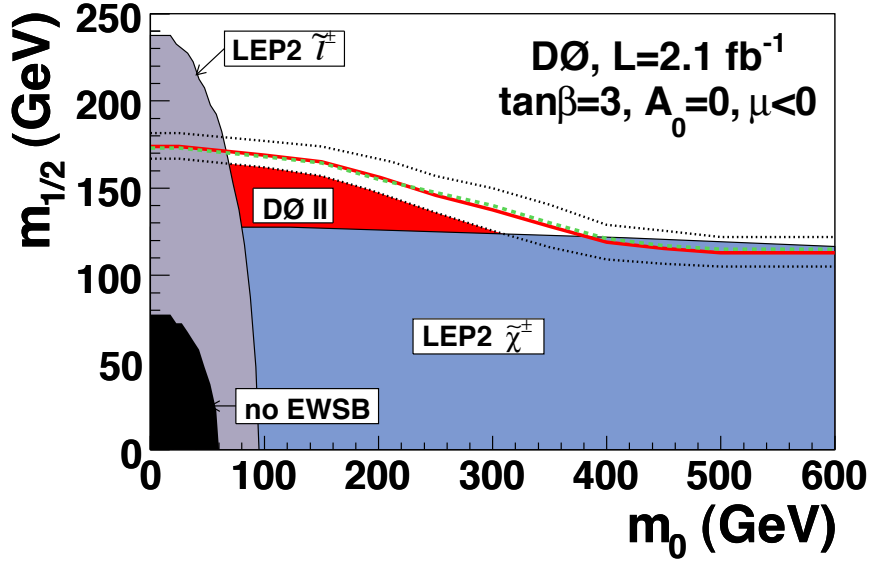
Figure 4: Region in the (m_0, m_{1/2}) plane excluded by the search for squarks and gluinos by D\O and by the searches for sleptons and charginos by the LEP experiments. The band at the edge of the excluded region represents the uncertainty associated with the scale and PDF choice, with the red curve corresponding to the nominal choice.
