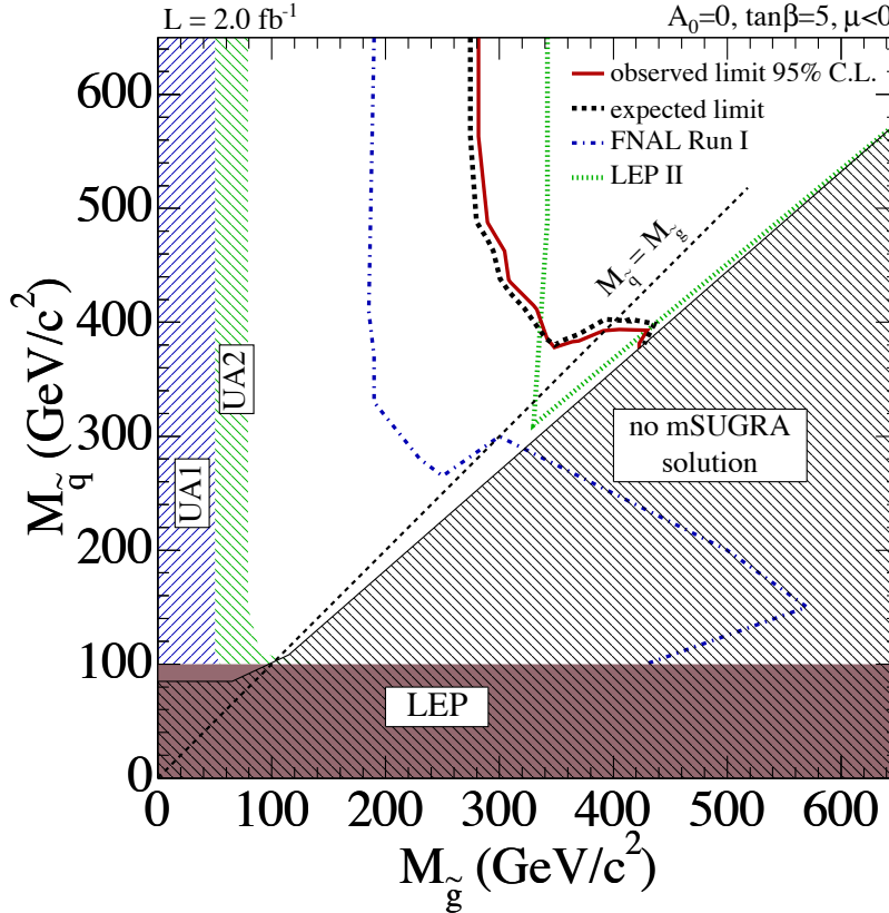
Figure 3: Region in the (m_{\tilde{g}}, m_{\tilde{q}}) plane excluded by CDF Run II and by earlier experiments.
