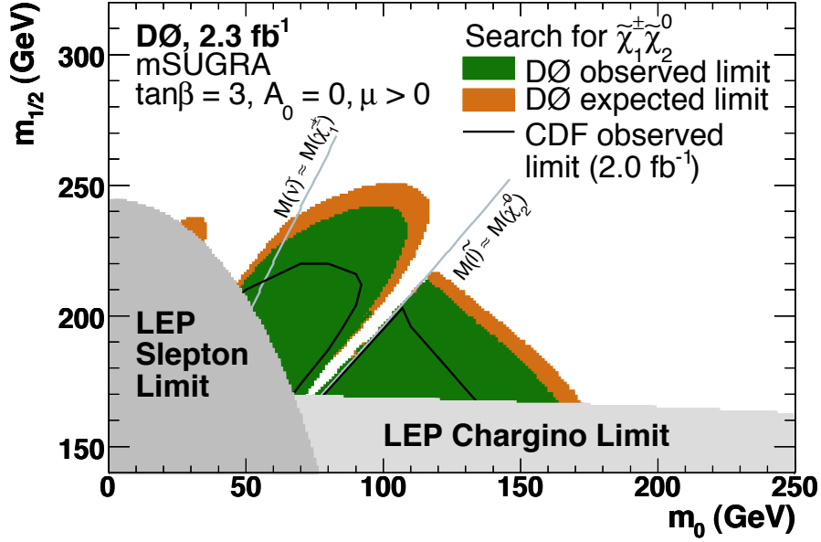
Figure 6: Regions in the (m_0, m_{1/2}) plane excluded by the D\emptyset search for trileptons and by the LEP experiments.
