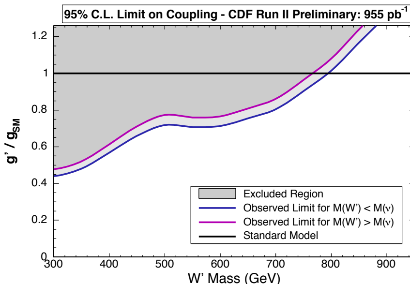
Figure 1: 95% CL exclusion limit from CDF [19] in the gauge coupling versus M_{W'} plane, using the t\bar{b} and t\bar{b} final states.
