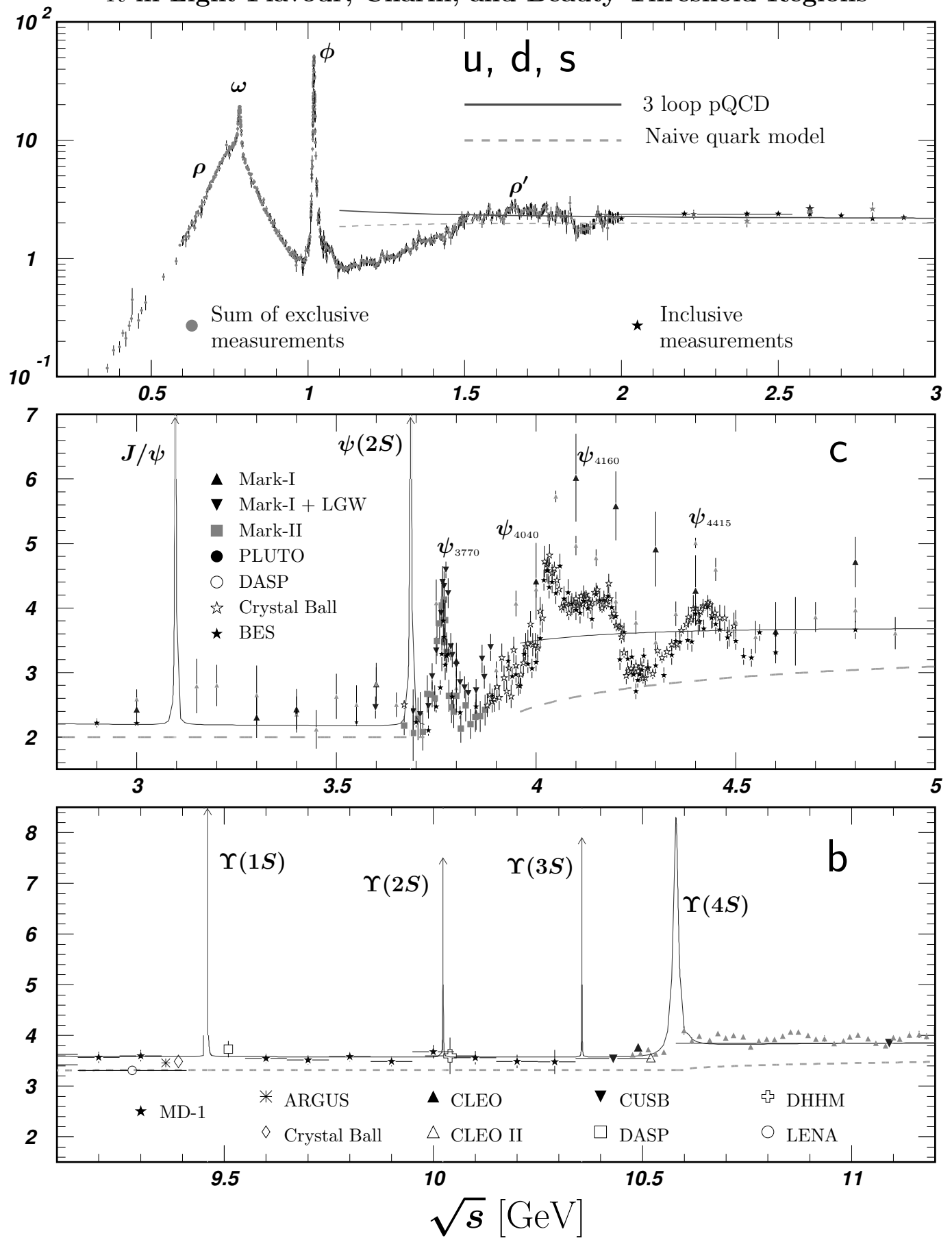
Figure 40.7: R in the light-flavour, charm, and beauty threshold regions. Data errors are total below 2 GeV and statistical above 2 GeV. The curves are the same as in Fig. 40.6. Note: CLEO data above \Upsilon(4S) were not fully corrected for radiative effects, and we retain them on the plot only for illustrative purposes with a normalization factor of 0.8. The full list of references to the original data and the details of the R ratio extraction from them can be found in [arXiv:hep-ph/0312114]. The computer-readable data are available at http://pdg.ihep.su/xsect/contents.html (Courtesy of the COMPAS(Protvino) and HEPDATA(Durham) Groups, August 2005.)
