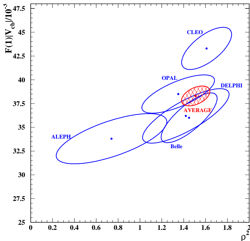
Figure 1: The error ellipses for the corrected measurements and world average for \mathcal{F}(1)|V_{cb}| vs \rho^2 . The ellipses are the product between the 1\sigma error of \mathcal{F}(1)|V_{cb}| , \rho^2 , and the correlation between the two. Consequently the ellipses correspond to about 37% CL.
