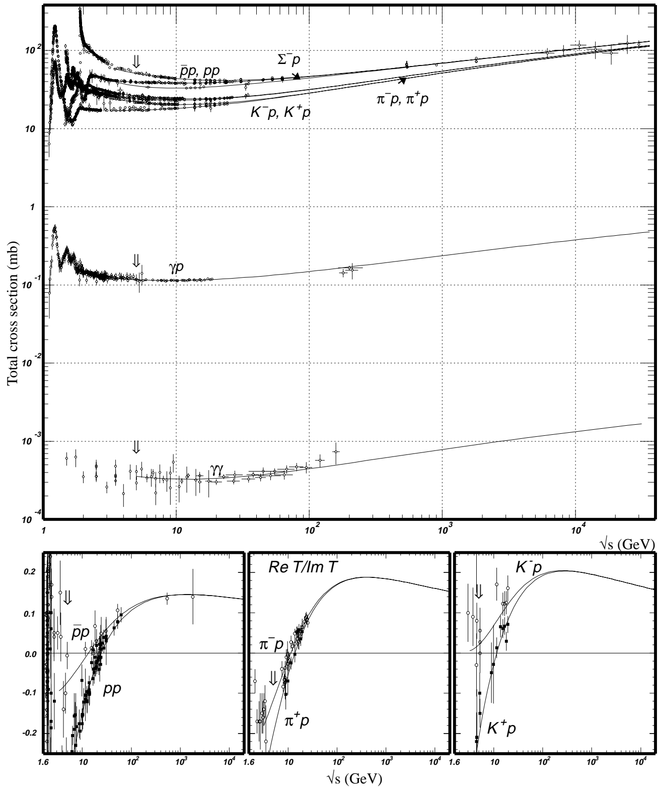
Figure 39.11: Summary of hadronic, \gamma p , and \gamma\gamma total cross sections, and ratio of the real to imaginary parts of the forward hadronic amplitudes. Corresponding computer-readable data files may be found at http://pdg.lbl.gov/xsect/contents.html (Courtesy of the COMPAS group, IHEP, Protvino, Russia, July 2001.)
