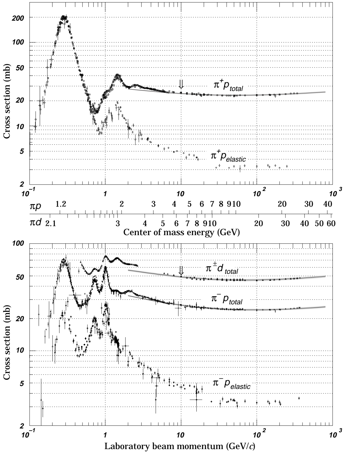
Figure 38.11: Total and elastic cross sections for \pi^\pm p and \pi^\pm d (total only) collisions as a function of laboratory beam momentum and total center-of-mass energy. Corresponding computer-readable data files may be found at http://pdg.lbl.gov/xsect/contents.html (Courtesy of the COMPAS Group, IHEP, Protvino, Russia, August 1999.)
