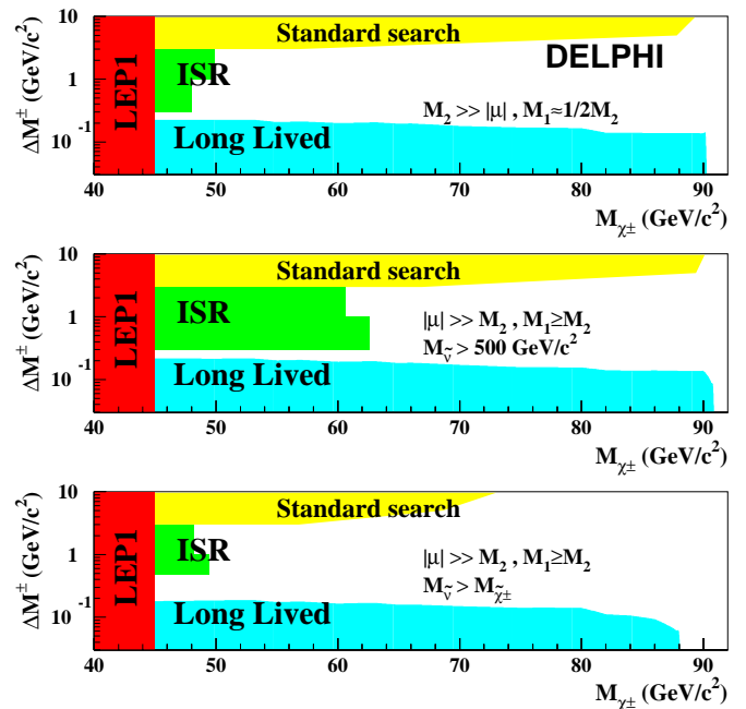
Figure 1: Ranges of excluded chargino and neutralino masses, for very small \Delta M , from DELPHI [10].
