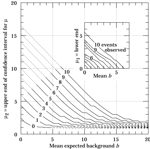
Figure 28.5: 90% confidence intervals [\mu_1, \mu_2] on the number of signal events as a function of the expected number of background events b . For example, if the expected background is 8 events and 5 events are observed, then the signal is 2.60 or less with 90% confidence. Dotted portions of the \mu_2 curves on the upper left indicate regions where \mu_1 is non-zero (as shown by the inset). Dashed portions in the lower right indicate regions where the probability of obtaining the number of events observed or fewer is less than 1%, even if \mu = 0 . Horizontal curve sections occur because of discrete number statistics. Tables showing these data as well as the CL = 68.27%, 95%, and 99% results are given in Ref. 13. There is considerable discussion about the behavior of the intervals when the number of observed events is less than the expected background; see Ref. 5
