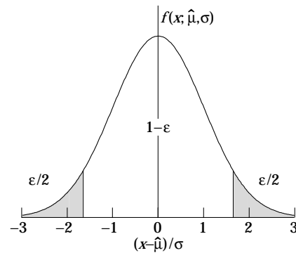
Figure 28.2: Illustration of a symmetric 90% confidence interval (unshaded) for a measurement of a single quantity with Gaussian errors. Integrated probabilities, defined by \varepsilon , are as shown.
