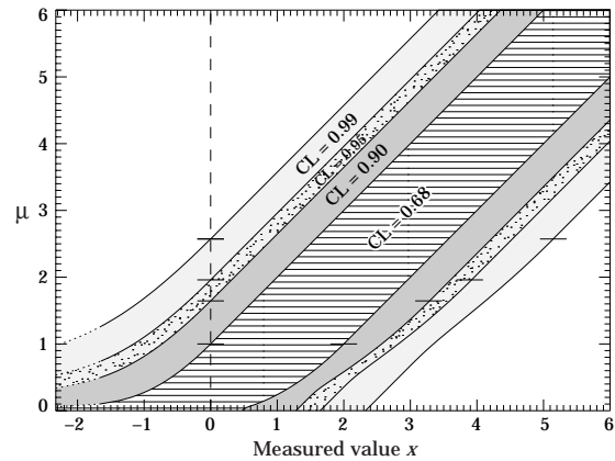
Figure 28.4: Plot of 99%, 95%, 90%, and 68.27% (“one \sigma ”) confidence intervals (using the unified approach as in Ref. 13) for a physical quantity \mu based on a Gaussian measurement x (in units of standard deviations), for the case where the true value of \mu cannot be negative. The curves become straight lines above the horizontal tick marks. The probability of obtaining an experimental value at least as negative as the left edge of the graph ( x = -2.33 ) is less than 1%. Values of x more negative than -1.64 (dotted segments) are less than 5% probable, no matter what the true value of \mu .
