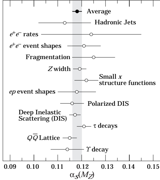
Figure 9.1: Summary of the value of \alpha_s(M_Z) from various processes. The values shown indicate the process and the measured value of \alpha_s extrapolated up to \mu = M_Z . The error shown is the total error including theoretical uncertainties.
